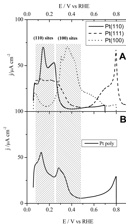
Figure 3. Voltammetric profiles of the Pt basal planes (A) to compare their site distribution with those obtained with a polyoriented platinum electrode (B) in 0.1 M HClO 4 . Scan rate, 50 mV s -1 .
