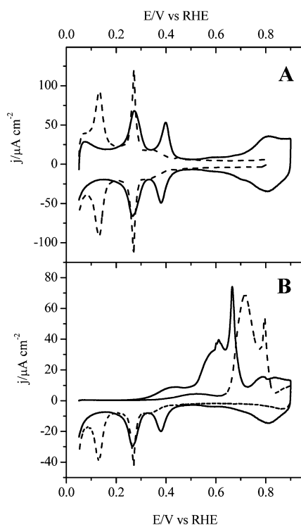
Figure 7. (A) Voltammetric profiles of a polycrystalline electrode in 0.1 M NaOH (full line) and 0.5 M H 2 SO 4 (dashed line) (scan rate, 50 mV s -1 ). (B) CO stripping voltammograms in 0.1 M NaOH (full line) and 0.5 M H 2 SO 4 (dashed line) (scan rate, 20 mV s -1 ).
